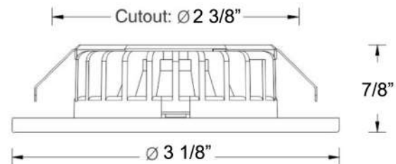
RECESSED MOUNTING
