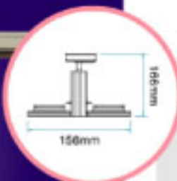
Model: LSP-1172/HT-303
