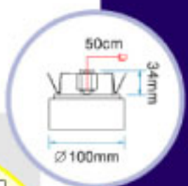
Model: LDL-905A1
