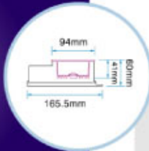
Model: ODL-C01/LDL-AC16
