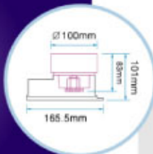
Model: ODL-905A1/LDL-AC15
