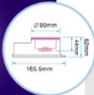
Model: ODL-905A/LDL-AC15
