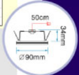
Model: LDL-905A
